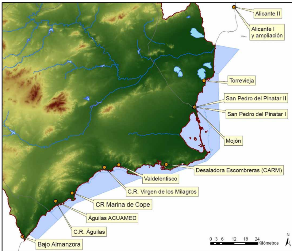
Figure 9 | Seawater desalination plants recorded in the Segura River Basin District Planning process. Source: SRBD. Ministry of Agriculture and Fisheries, Food and Environment.
